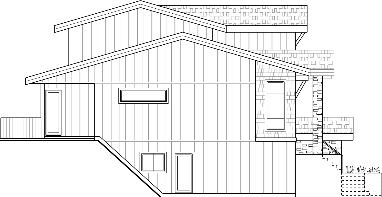
LEFT ELEVATION
